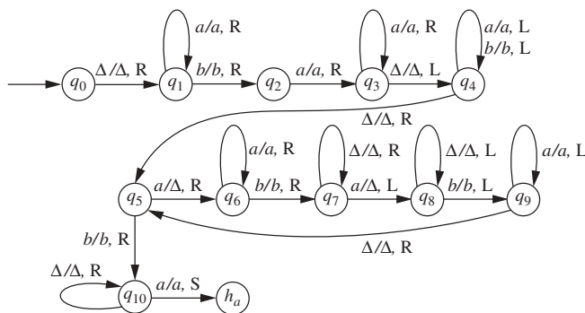
Figure 7.8 | A Turing machine accepting \{a^i b a^j \mid 0 \leq i < j\} .
