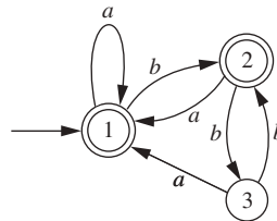
Figure 3.33 | An FA for which we want an equivalent regular expression.
