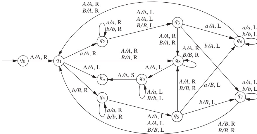
Figure 7.11 | A Turing machine computing the reverse function.
