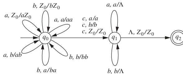
Figure 5.5 | A transition diagram for a PDA accepting SimplePal .
