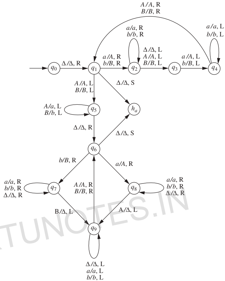
Figure 11.3 | A Turing machine accepting \{xx \mid x \in \{a, b\}^*\} .
