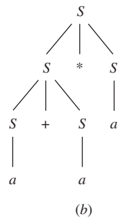
Figure 4.22 | Two derivation trees for a + a * a in Example 4.2.
