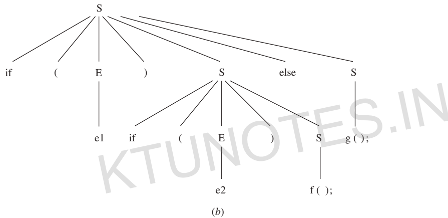
Figure 4.21 | Two possible interpretations of a dangling else .
