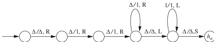
Figure 7.29 | An NTM to generate a string of two or more 1's.
